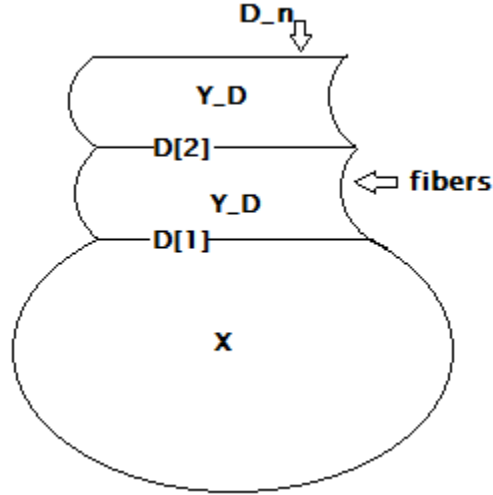
Figure 4.1: The singular manifold X[n] .
